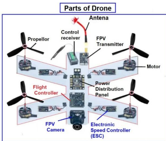
Figure 5. Parts of a Drone
